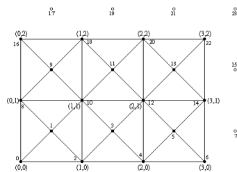
Figure 3.70: Triangle arrangement for a 4x3 image
