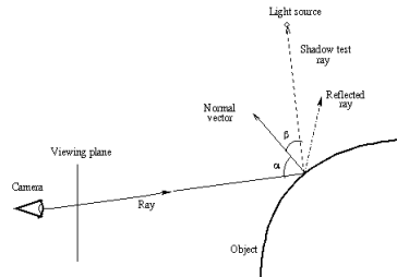
Figure 3.69: The basic raytracing algorithm
